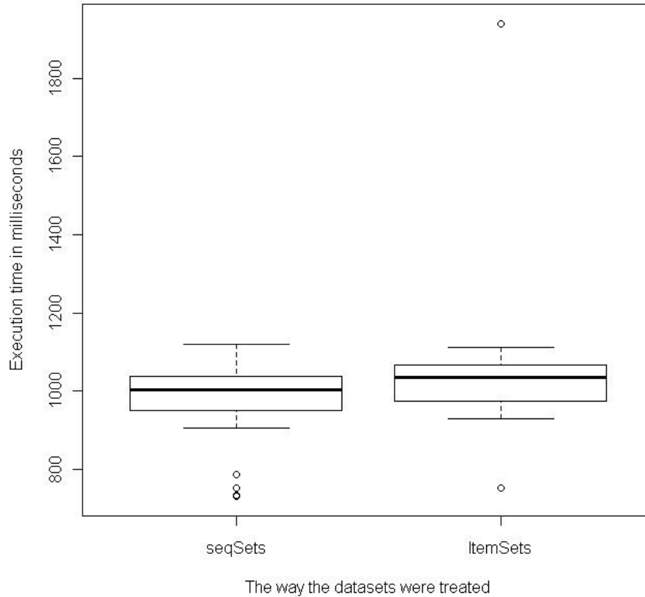
Figure 5.9: Time taken to build the FP trees in experiment 1
